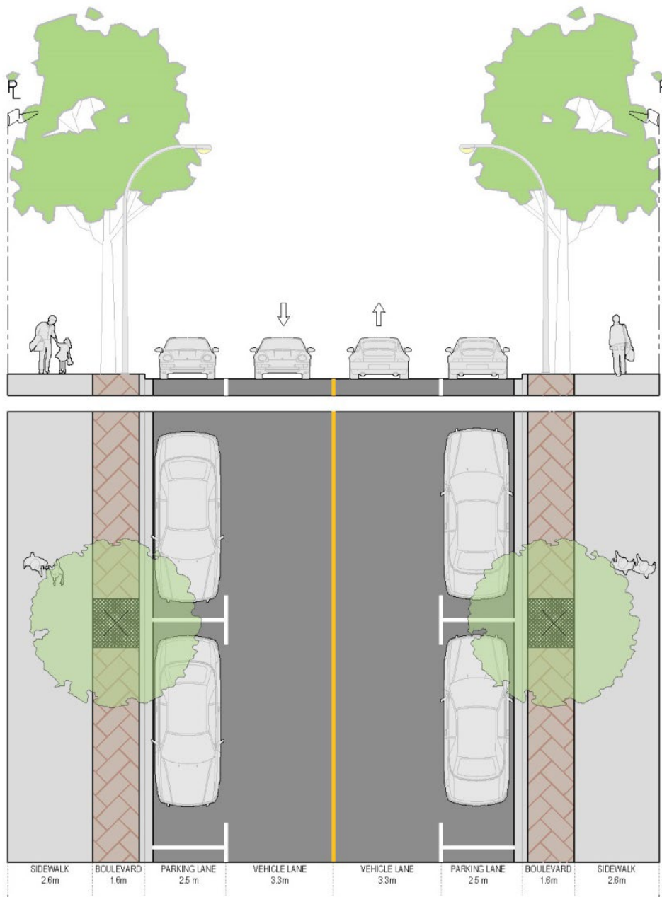
Figure 44 – Cross Section: 20.0m Local
