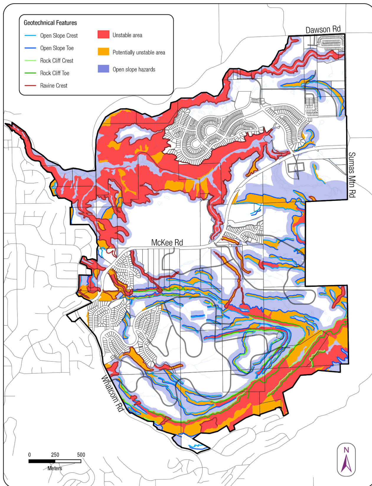
Map 5. Geotechnical Features
